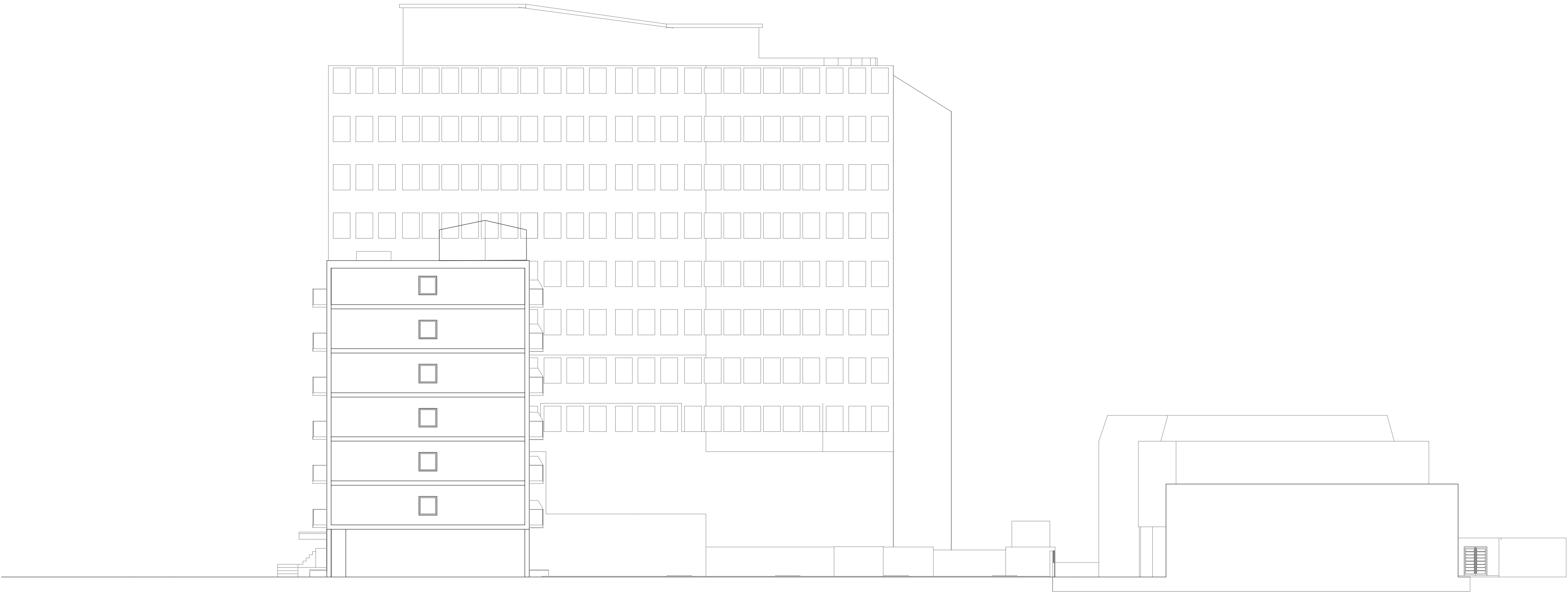
Existing North Elevation - 1:200
